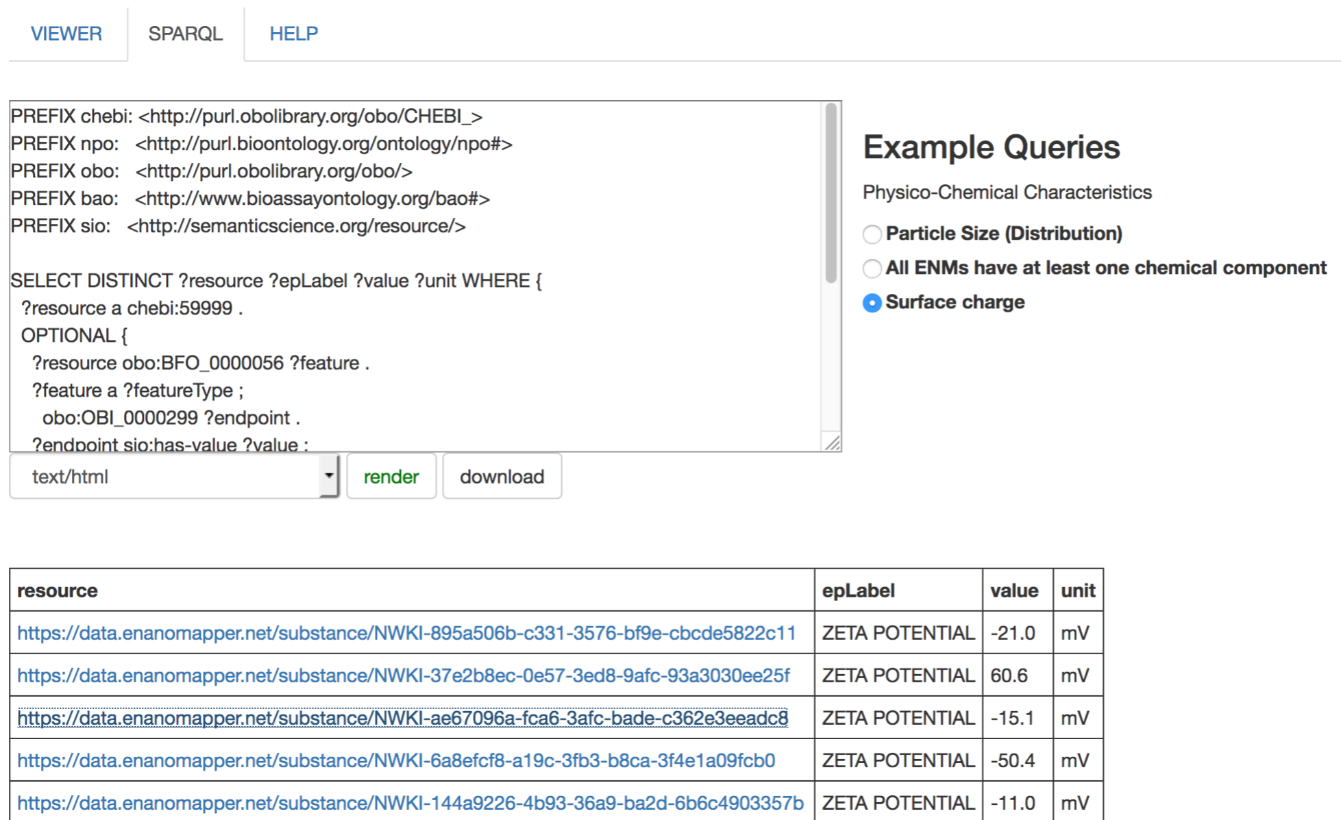
Figure 6: SPARQL interface. Select one of the physico-chemical characteristics examples.
